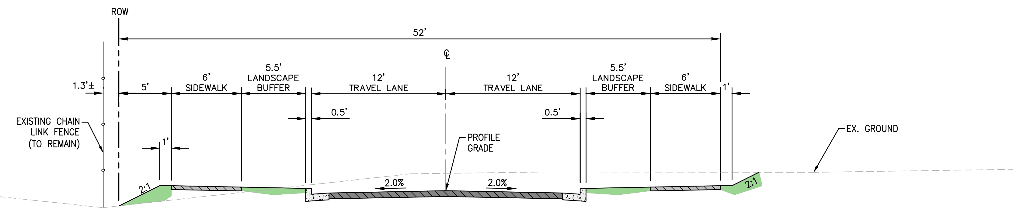
4 OPTION 1 (7TH-4TH) 5' BUFFER & 12' LANES SCALE: NTS
