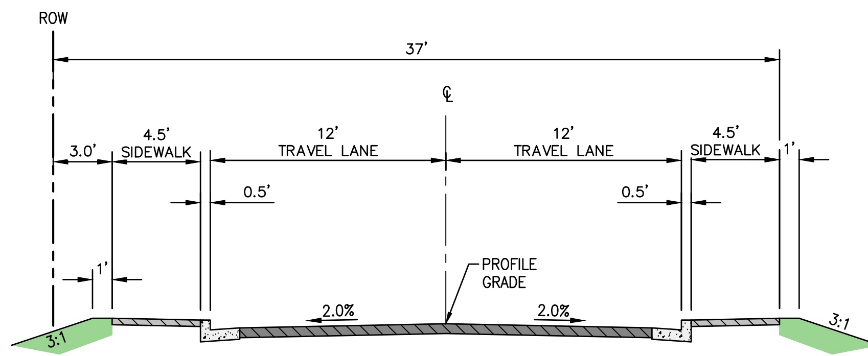
1 OPTION 1 (10TH-7TH) 12' LANES & 4.5' SIDEWALKS SCALE: NTS
