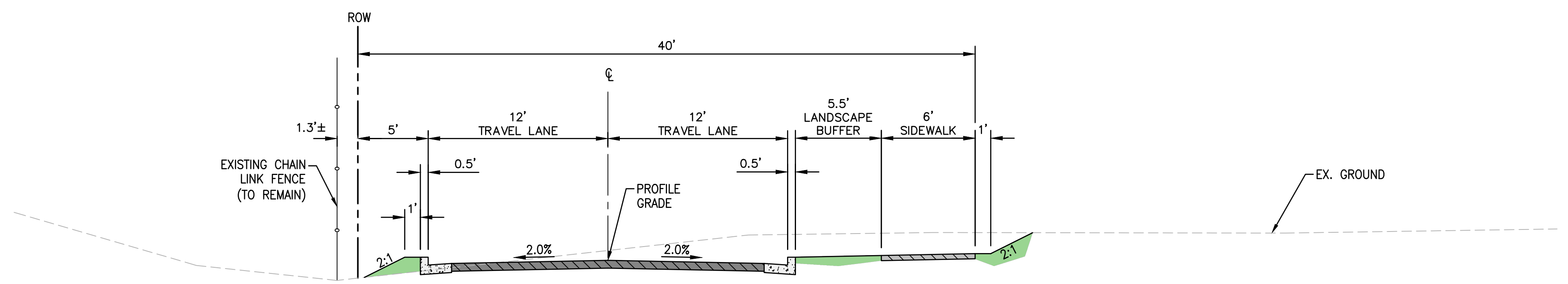
7 OPTION 3 (7TH-4TH) WITHOUT NORTH SIDEWALK SCALE: NTS
