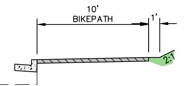
6 OPTION 2 (7TH-4TH) CURB-TIGHT BIKEPATH SCALE: NTS
