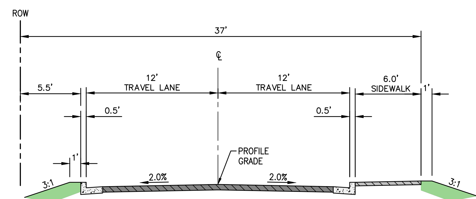
3 OPTION 3 (10TH-7TH) 12' LANES, SOUTH SIDEWALK SCALE: NTS
