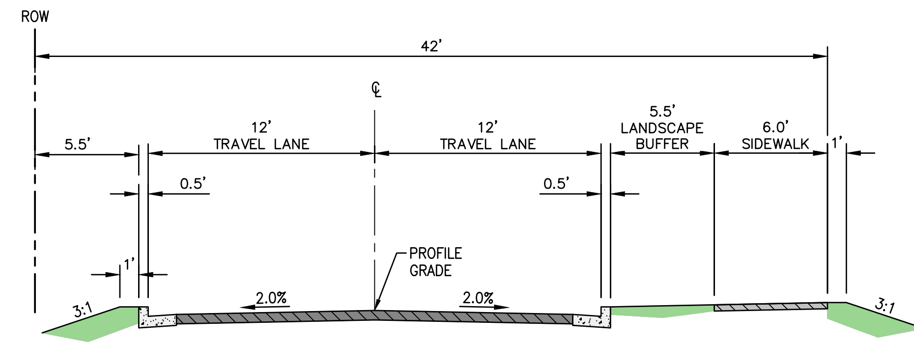
2 OPTION 2 (10TH-7TH) 12' LANES, SOUTH BUFFER & SIDEWALK SCALE: NTS
