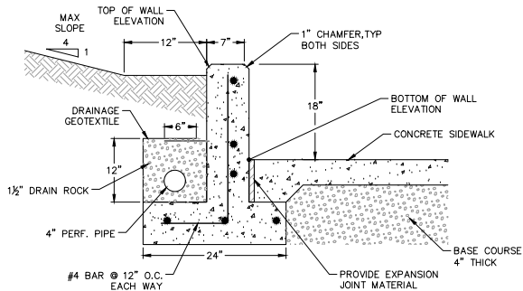
NOTES: 1. PROVIDE SCORE AND CONTRACTION JOINTS PER DETAIL 11/C6.1. 9 CONCRETE RETAINING WALL SCALE: NTS
