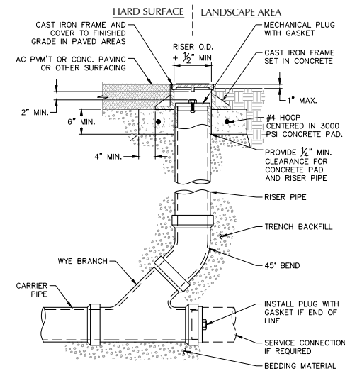
NOTES: 1. CAST IRON FRAME AND COVER SHALL MEET H-20 LOAD REQUIREMENT. 2. FOR CARRIER PIPE SIZE 6" Ø AND LESS, PROVIDE RISER PIPE SIZE TO MATCH CARRIER PIPE. 3. FOR CARRIER PIPE SIZE 8" Ø AND LARGER, RISER PIPE SHALL BE 6" Ø. 4. RISER PIPE MATERIAL TO MATCH CARRIER PIPE MATERIAL. 5 STANDARD CLEANOUT (COTG) SCALE: NTS
