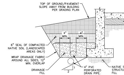
NOTES: 1. LAY PERFORATED DRAIN PIPE ON MIN. 0.5% GRADIENT, WIDENING EXCAVATION AS REQUIRED. MAINTAIN PIPE ABOVE 2:1 SLOPE AS SHOWN. 2. CONNECT TO FOUNDATION DRAIN STUBOUT SHOWN ON PLANS. 4 PERIMETER FOUNDATION DRAIN SCALE: NTS
