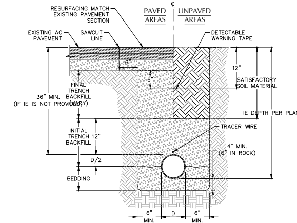
10 TYPICAL PIPE BEDDING AND BACKFILL SCALE: NTS
