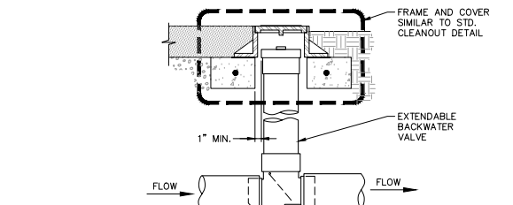
NOTES: 1. EXTENDABLE BACKWATER VALVE TO BE MANUFACTURED BY CLEAN CHECK OR APPROVED EQUAL AND SHALL BE INSTALLED PER MANUFACTURER'S RECOMMENDATIONS. 8 EXTENDABLE BACKWATER VALVE SCALE: NTS
