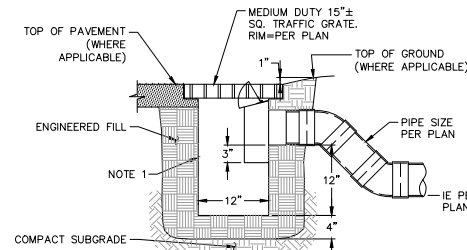
NOTE: 1. TO GAGE STEEL PLATE, BITUMINOUS COATED, AS MANUFACTURED BY GIBSON STEEL BASINS OR APPROVED EQUAL. 3 TRAPPED AREA DRAIN SCALE: NTS
