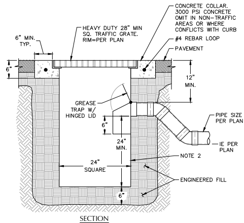
NOTES: 1. CONTRACTOR TO WIDEN EXCAVATION AS REQUIRED TO OBTAIN COMPACTION WITH CONTRACTORS COMPACTION EQUIPMENT. 2. 1/4" STEEL PLATE, BITUMINOUS COATED, AS MANUFACTURED BY GIBSON STEEL BASINS OR APPROVED EQUAL. 5 TRAPPED CATCH BASIN SCALE: NTS
