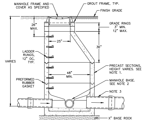
NOTES: 1. ALL PRECAST SECTIONS SHALL CONFORM TO REQUIREMENTS OF ASTM C-478. 2. MANHOLE BASE MAY BE PRECAST OR CAST IN PLACE. SEE STANDARD MANHOLE BASE DETAILS. 7/C7.02. 3. ALL CONNECTING PIPES SHALL HAVE FLEXIBLE, GASKETED AND UNRESTRAINED JOINT WITHIN 18" OF MANHOLE VAULT. 6 STANDARD MANHOLE SCALE: NTS
