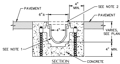
NOTES: 1. TRENCH DRAIN SHALL BE PRE-SLOPED 6" WIDE ZURN TRENCH DRAIN OR APPROVED EQUAL. 2. TRENCH DRAINS GRATE SHALL BE LOCKABLE HEAVY DUTY ADA TRENCH GRATE - CLASS C. 3. TRENCH SYSTEM SHALL BE INSTALLED PER MANUFACTURER'S INSTRUCTIONS. 4. PROVIDE BOTTOM OUTLET AT LOWPOINT PER MANUFACTURER DETAILS. 11 TRENCH DRAIN - 6 INCH WIDE SCALE: NTS
