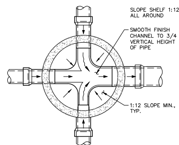
NOTES: 1. BASED MAY BE PRECAST OR CAST IN PLACE. 2. ALL PRECAST SECTIONS SHALL CONFORM TO REQUIREMENTS OF ASTM C-478. 3. CONCRETE SHALL BE COMMERCIAL GRADE. 4. CHANNELS SHALL BE CONSTRUCTED TO PROVIDE SMOOTH SLOPES AND RADII TO OUTLET PIPE. 5. EXTEND PIPE INTO MANHOLE AND GROUT SMOOTH. PIPE(S) MAY EXTEND 2" MAX BEYOND THE INTERIOR MANHOLE WALL. 7 MANHOLE BASE - STANDARD SCALE: NTS
