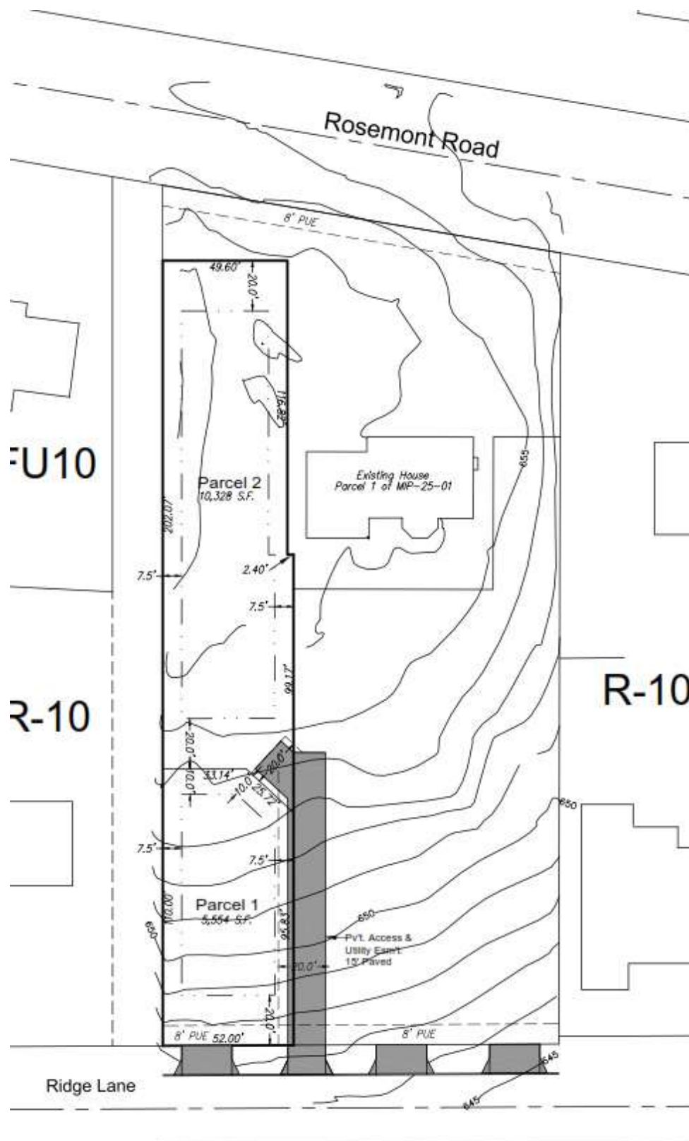
Site Plan
