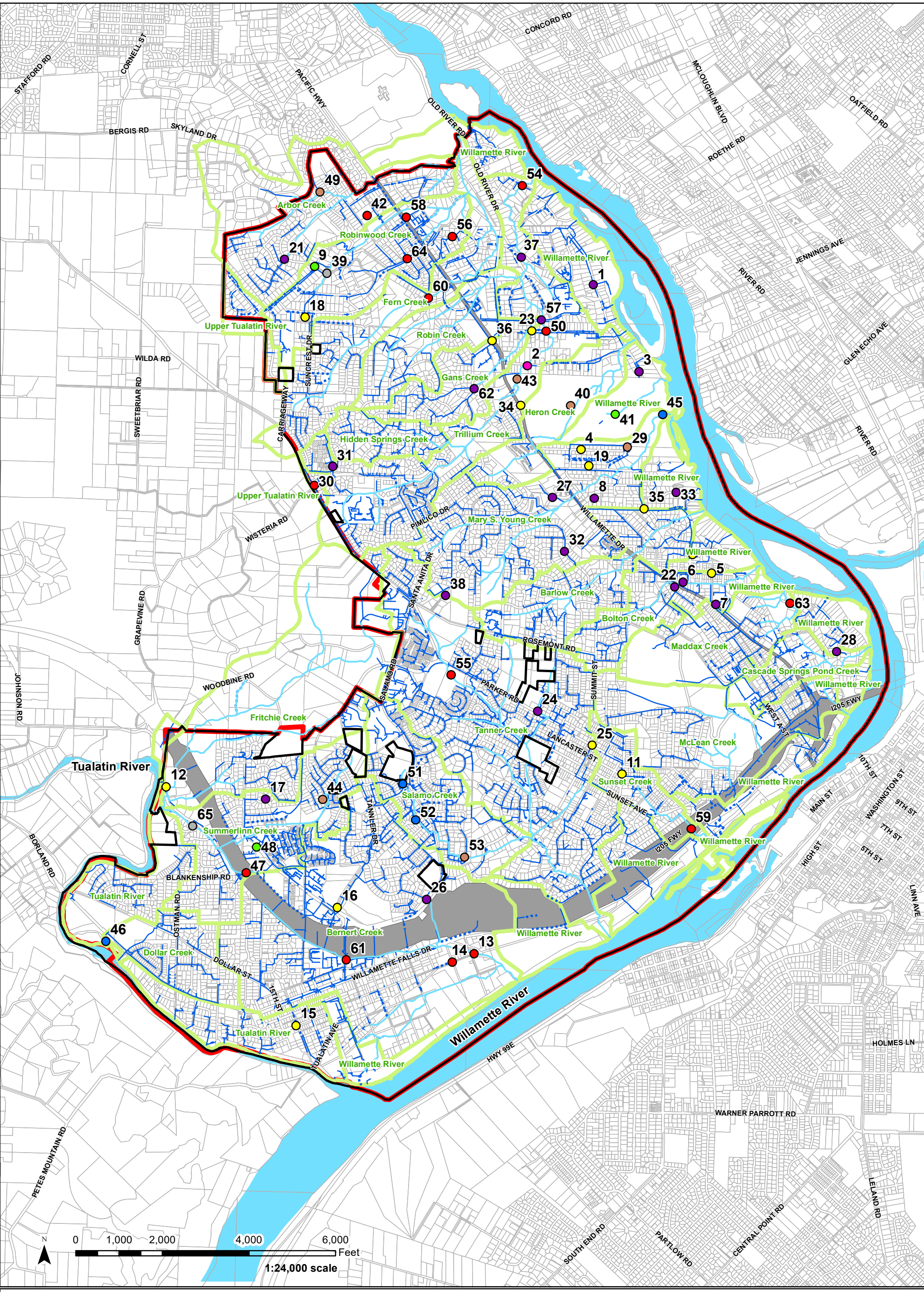
CITY OF WEST LINN, OREGON Storm Drainage and Sanitary Master Plan 2019 Figure 1: Storm Drainage Problem Areas
