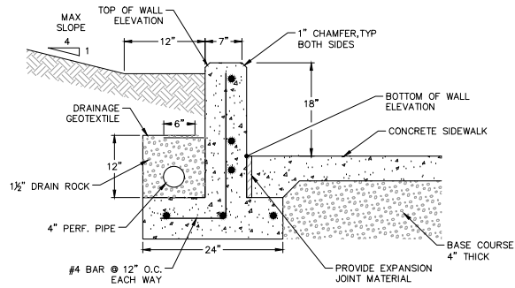
9 CONCRETE RETAINING WALL SCALE: NTS
