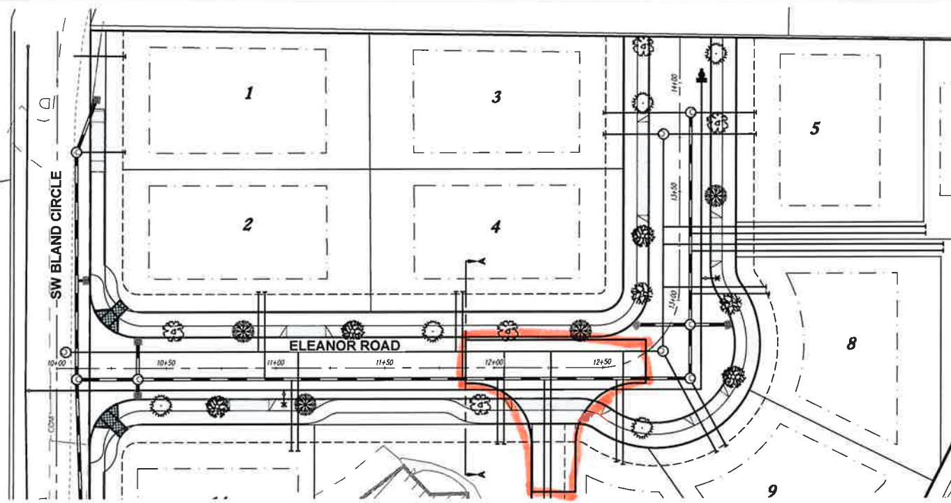
ELEANOR ROAD PLAN SCALE: 1"=30'
