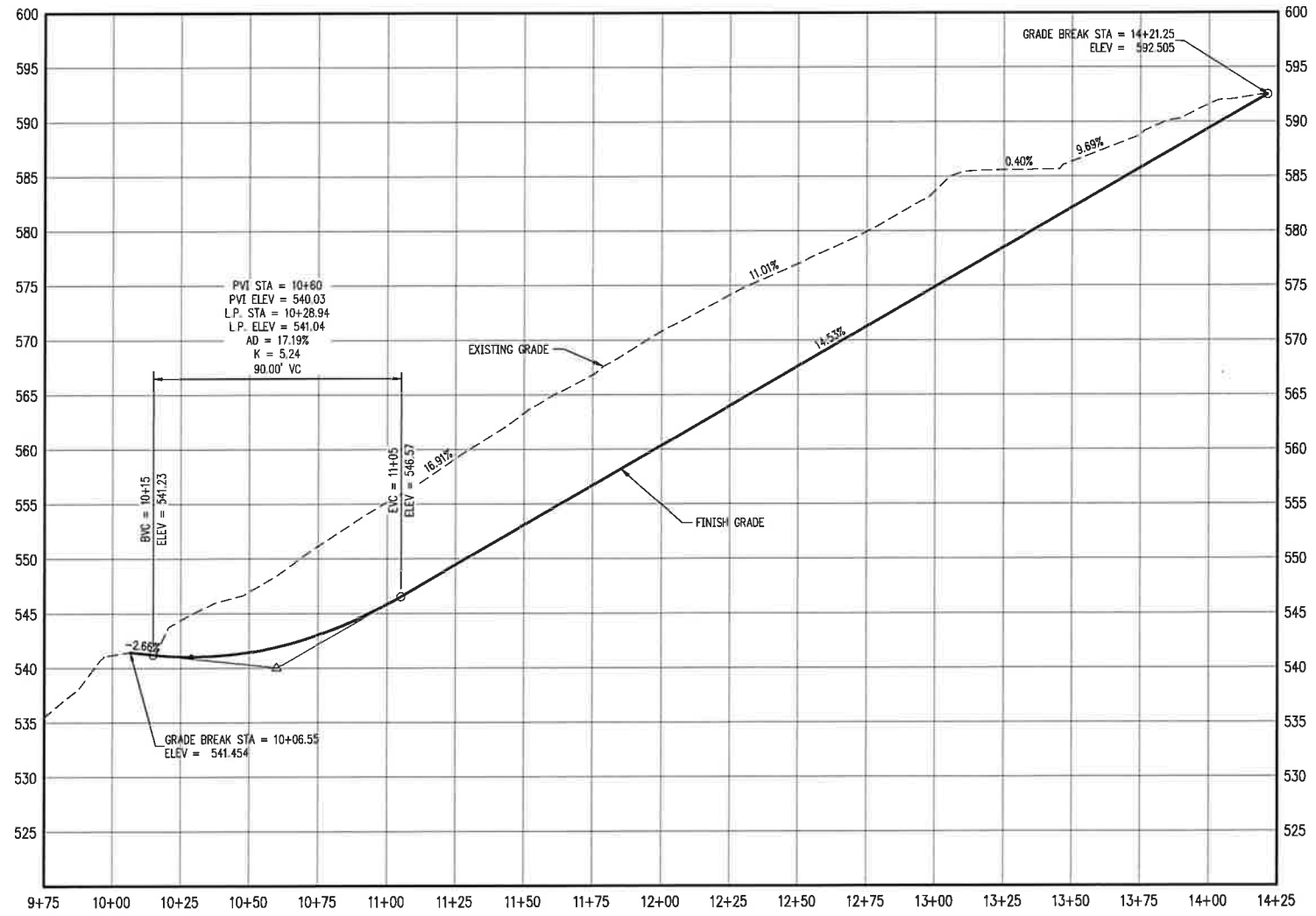
ELEANOR ROAD PROFILE SCALE: 1"=30' HORZ. 1"=7.5' VERT.
