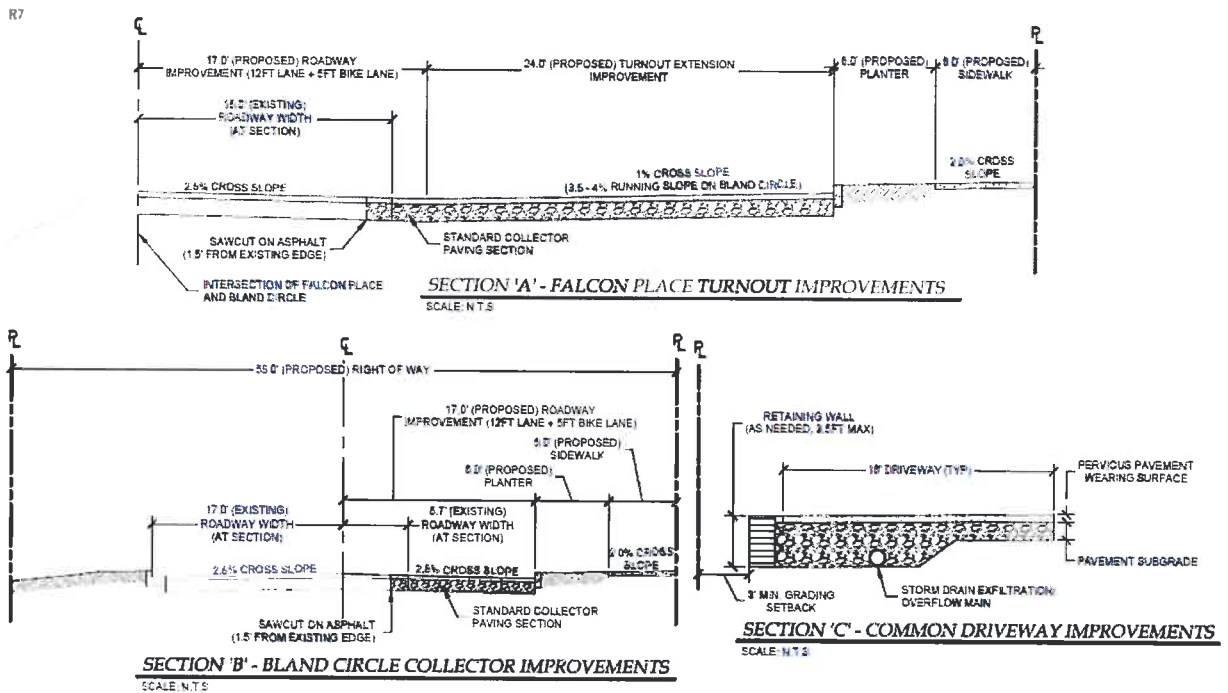
Figure 12: Proposed street cross sections
