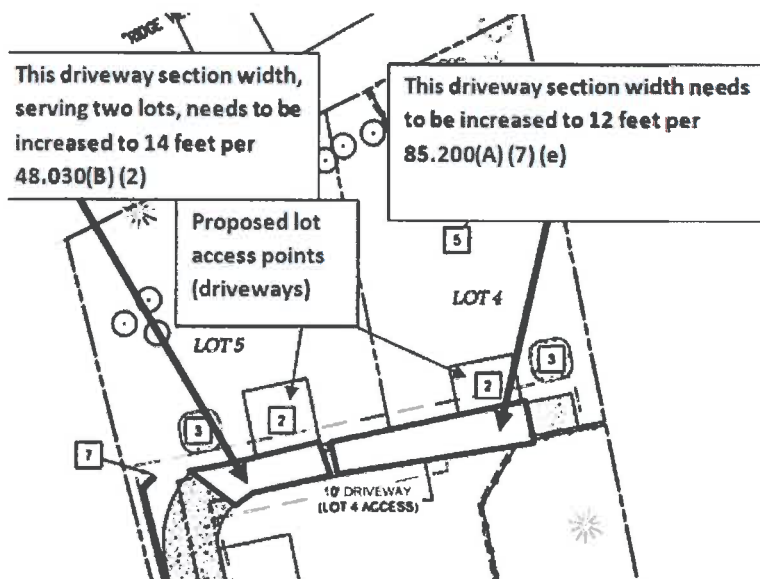
Figure 16: Required driveway widths
