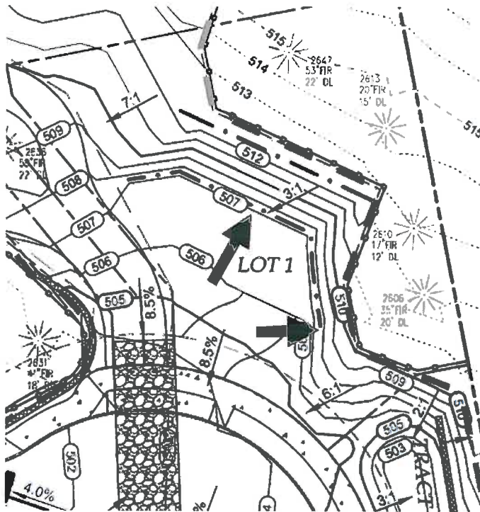
Figure 19: Grading plan for lot 1. The access driveway, the "eyebrow" and tree conservation easements dictate the grading plan.
