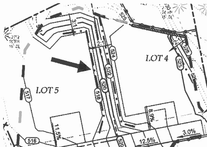
Figure 17: Grading between lots 4 and 5
