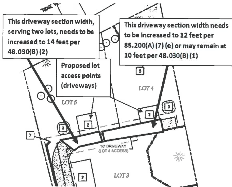
Figure 9: Required Driveway Width
