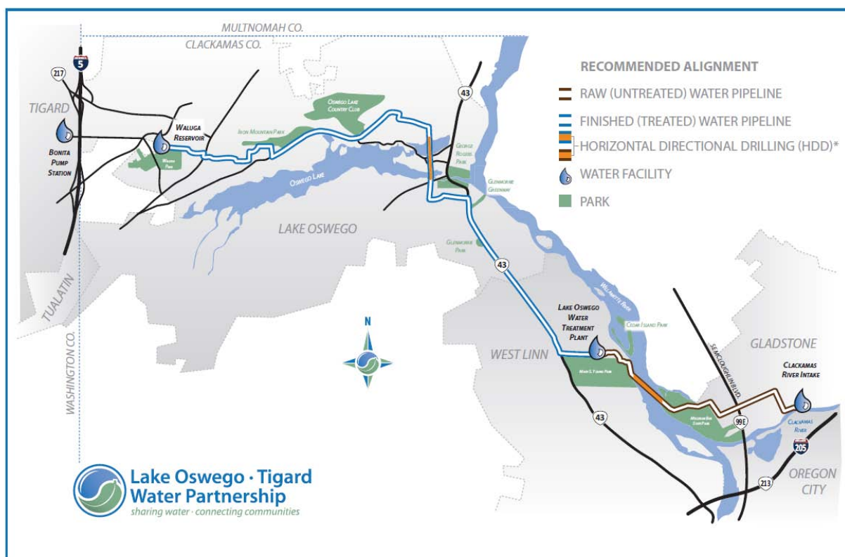
Figure 1.1: Lake Oswego-Tigard Water Supply Partnership Overview
