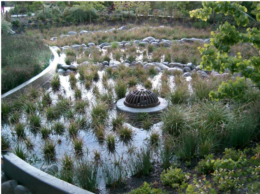
Exhibit 2-18: Glencoe School Infiltration Basin. See Appendix G.1 SW-140 for typical basin details.
